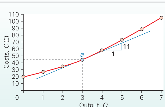
Figure A1.10 A total cost function: C = 20 + 5Q + Q^2
